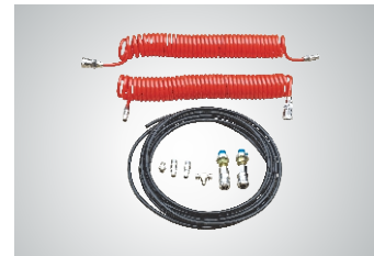
Optional airline kits. Easy and convenient installation with all models of rolling jacks with a pneumatic pump. Kits No.:PX004
