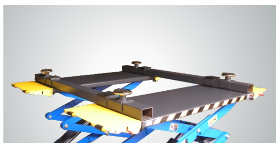
▲ Optional support bars & Kit. recommended for heavier vehicles with narrow frames. Kits No.:SX703
